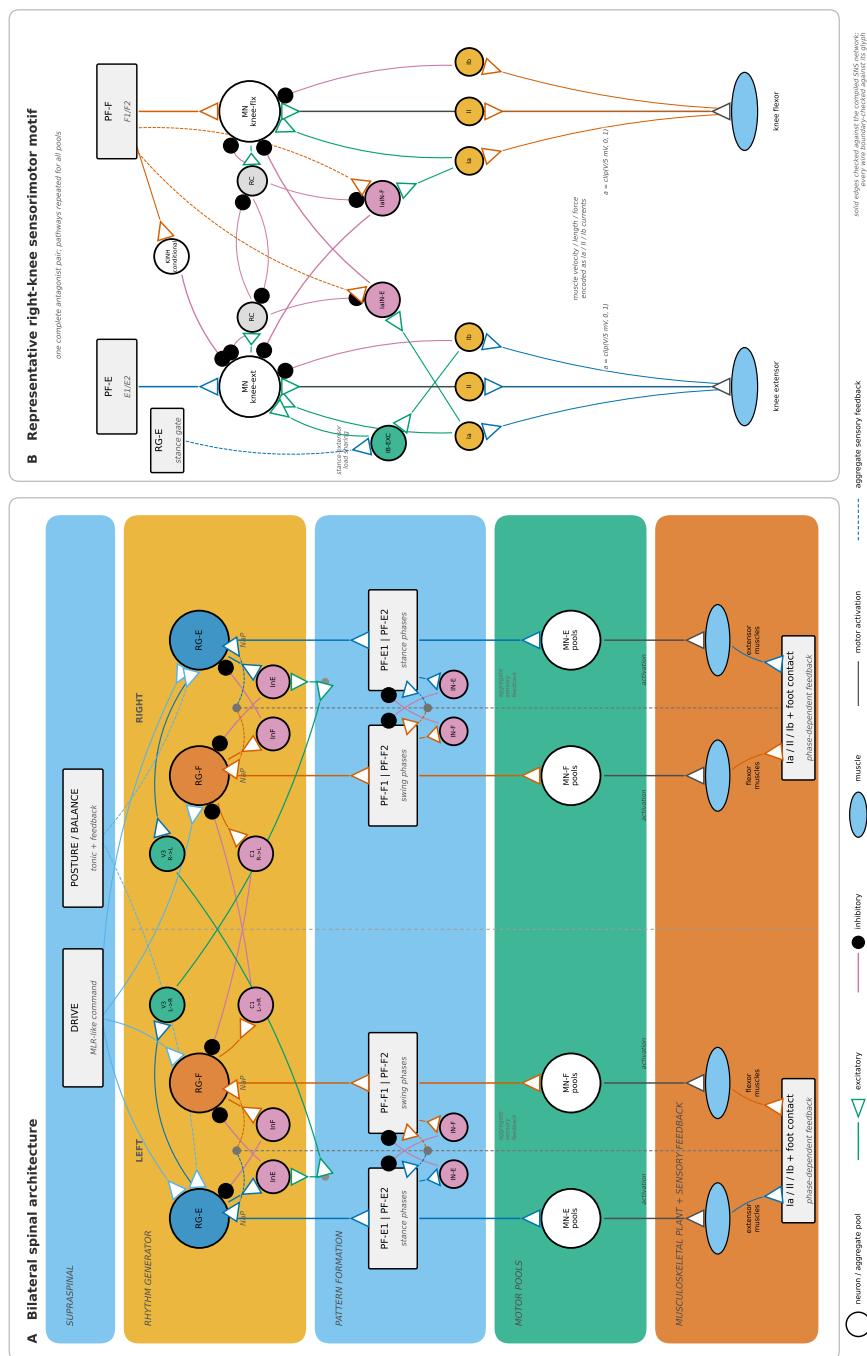
Figure 2.3: Locomotor circuit architecture synthesized from the literature. The bilateral organization combines rhythm-generation, pattern-formation, motoneuron, commissural, and proprioceptive pathways used across two-level CPG and neuromechanical models [???]. The detailed knee-control motif makes the reciprocal antagonist and sensory pathways explicit.
