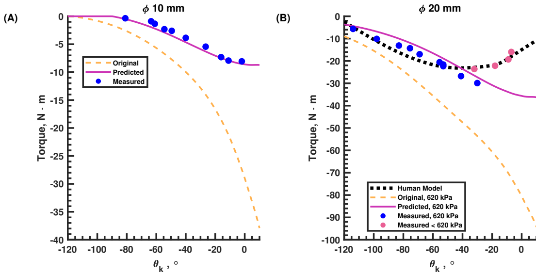
Figure 4.8: Biomimetic knee torque for (A) \phi 10 \text{ mm} l_0 = 41.5 \text{ cm} flexor BPA with a 21 mm artificial tendon. Blue dots show the measured torque values. Magenta line is the predicted torque using the improved BPA characterization and optimization from the previous sections. The dashed light orange line shows the torque predicted using only the improved BPA characterization. (B) \phi 20 \text{ mm} l_0 = 42.0 \text{ cm} flexor BPA with a 15 mm artificial tendon uses the same colors for 620 kPa results. Human values are given as a black dotted line. Due to the BPA exceeding the ultimate strength of the femur, torque measurements were taken at P < P_{620} to show the desired RoM is achievable. Results for torque measurements at 560 kPa, 421 kPa, 325 kPa and 281 kPa (from left to right, respectively), are shown as pink dots.
