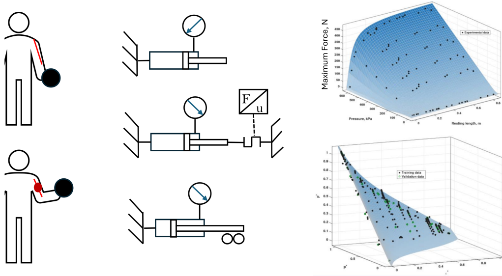
Figure 2.1: Overview of the BPA force-characterization study. Biological-muscle inspiration and the laboratory test apparatus lead to measured force-length-pressure data and fitted force surfaces used for actuator and robot design.
