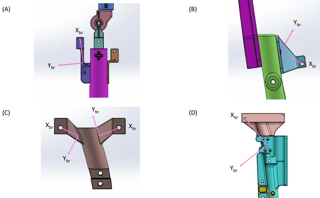
Figure 3.5: Bracket frame orientations for: (A) flexor configuration on the pinned knee, (B) extensor configuration on the pinned knee, (C) flexor and extensor configurations on the biomimetic knee with \phi 10 mm BPAs, and (D) flexor configuration on the biomimetic knee with the \phi 20 mm BPA.
